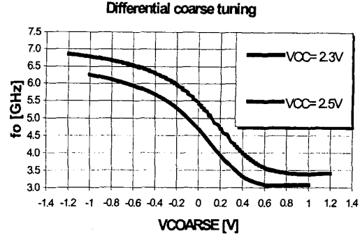
Fig.7: COARSE tuning curve @ VREPLICA=2.3V
