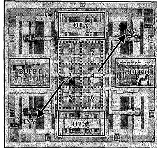
Fig.10: VCO chip photo
